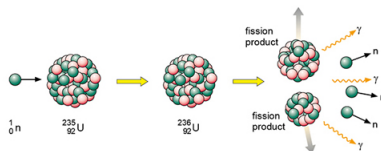
Figure: The example of the fission of Uranium-235
